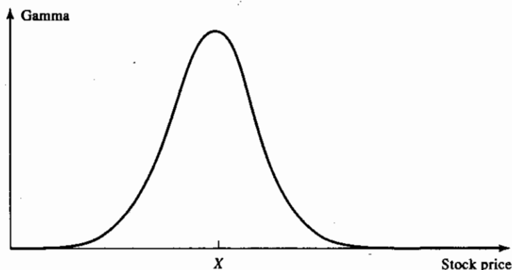
Figure 15.9 Variation of gamma with stock price for an option
