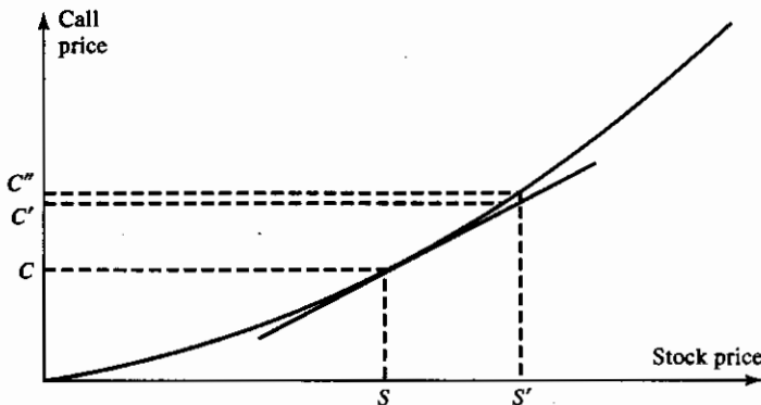
Figure 15.7 Hedging error introduced by curvature, or gamma
