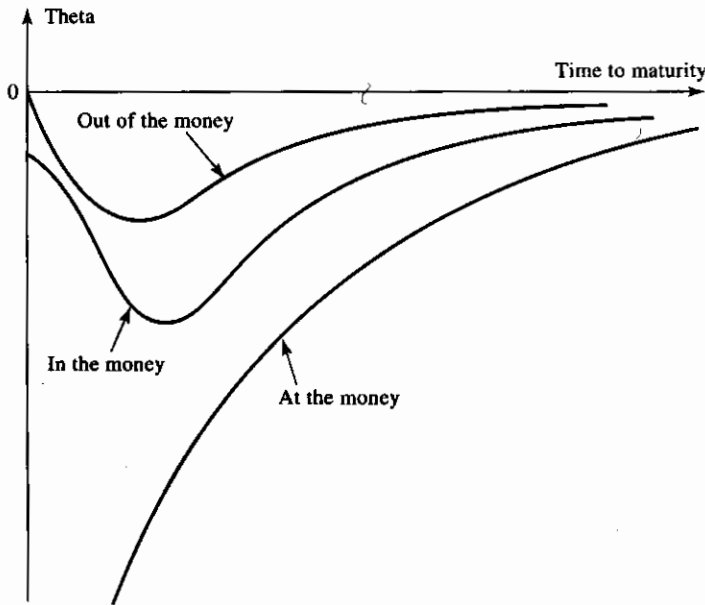
Figure 15.6 Typical patterns for variation of theta of a European call option with time to maturity
