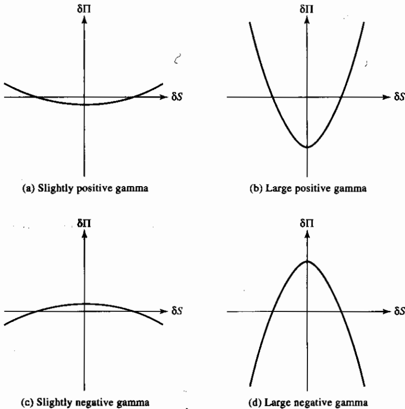
Figure 15.8 Alternative relationships between \delta\Pi and \delta S for a delta-neutral portfolio: (a) slightly positive gamma, (b) large positive gamma, (c) slightly negative gamma, and (d) large negative gamma
