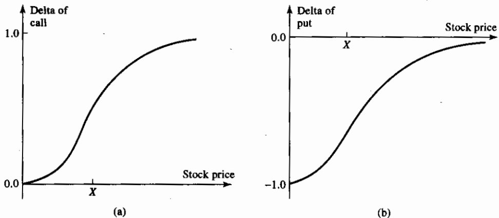
Figure 15.3 Variation of delta with stock price: (a) call option and (b) put option on a non-dividend-paying stock
